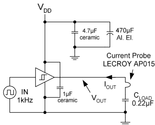
Figure 44. Quasi-Static I_{OUT} / V_{OUT} Test Circuit
