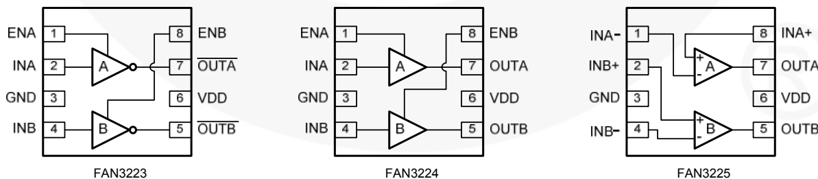
Figure 1. Pin Configurations
