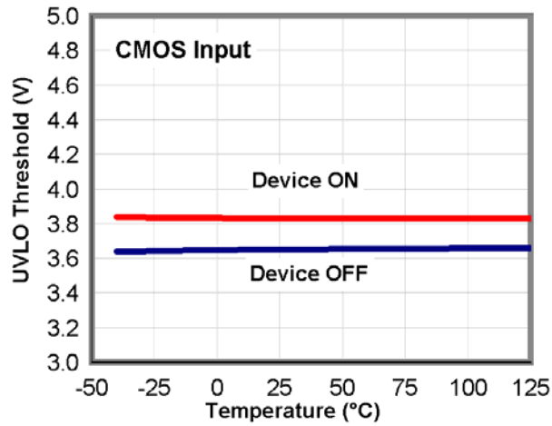
Figure 25. UVLO Thresholds vs. Temperature
