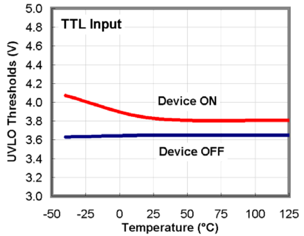
Figure 26. UVLO Threshold vs. Temperature
